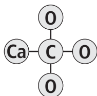
\text{CaCO}_3
