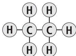
\text{C}_2\text{H}_6
