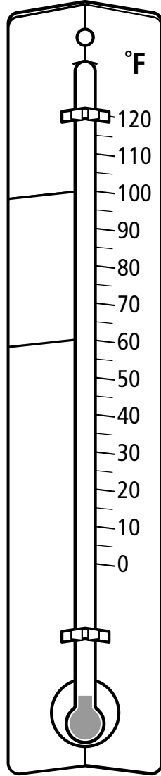
Dew formed
