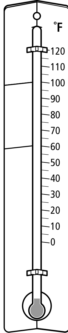
Frost formed
