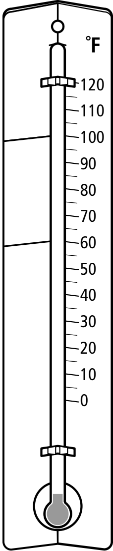
Start
