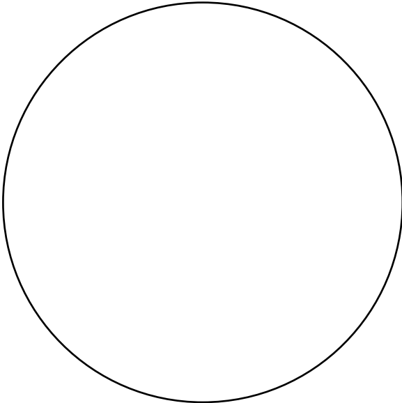
Full Moon
