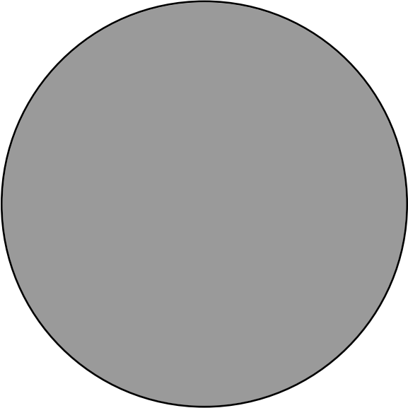
New Moon
